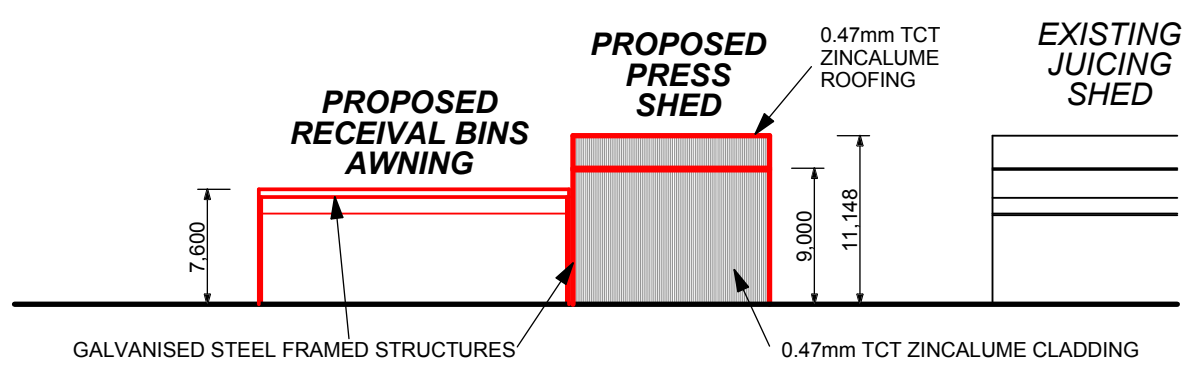
ELEVATION H - H
